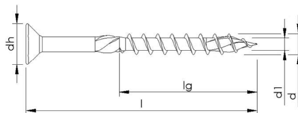
Part thread without variation, with shank ribs and milling ribs
