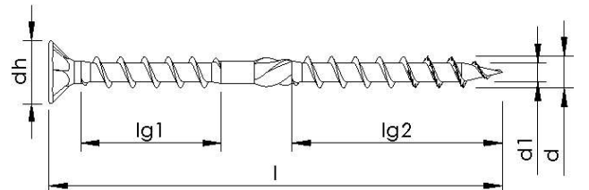
Secondary thread without variation, with shank ribs, with toothed tip
